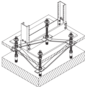
Rack with 3"(80 mm) channel shown
