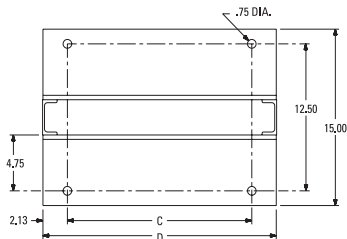
Top View of Base Angle
