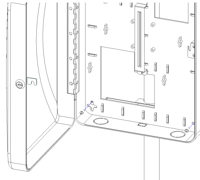
Figure 3 - Bottom Speaker Mount Bracket Install
